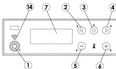
Fig. 6 - Betjeningspanel (wi-fi)
